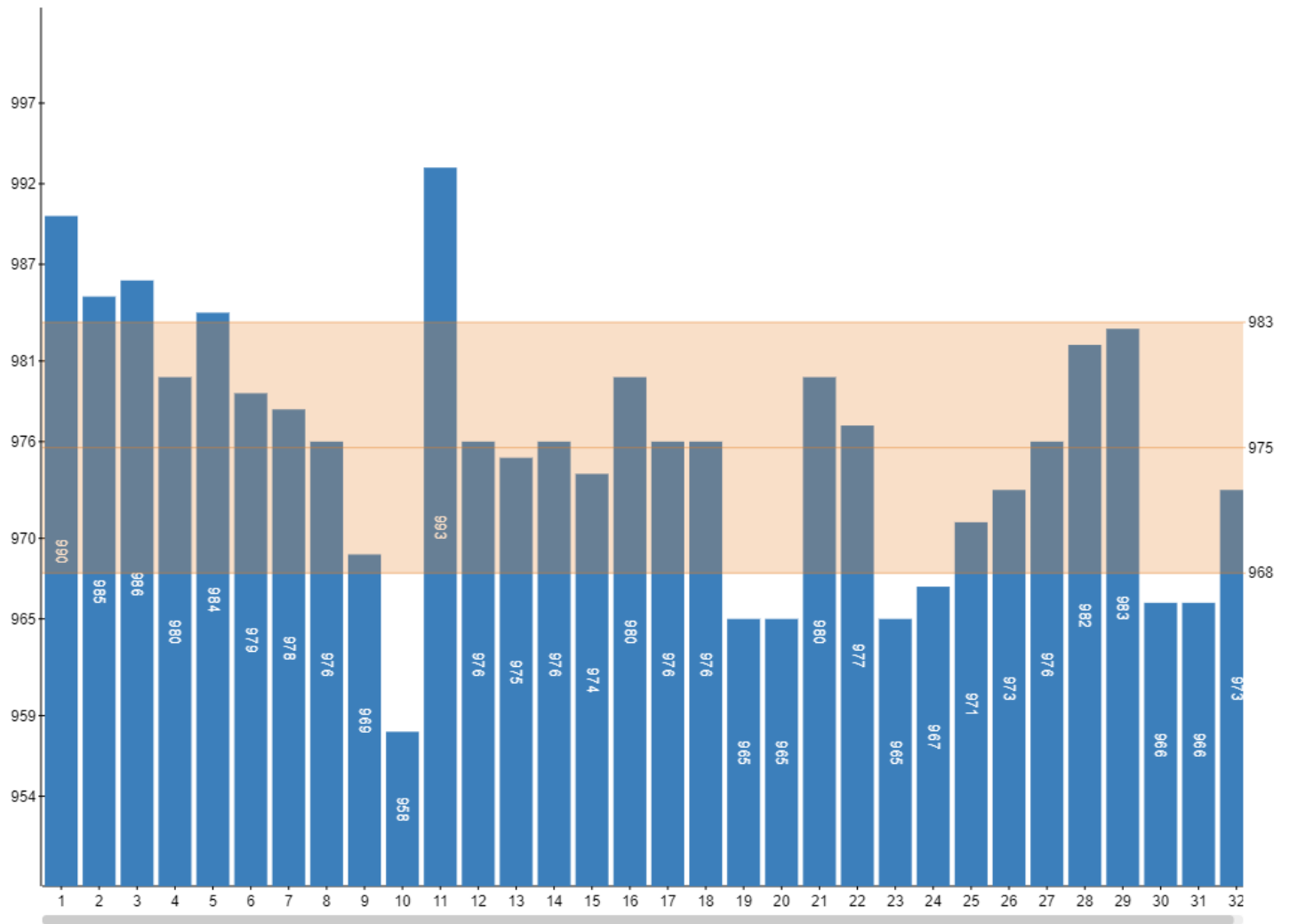
Standard Deviation
